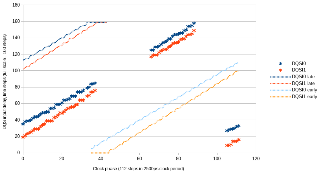
Measured (marginal) and calculated (optimal) DQS input delay vs phase
